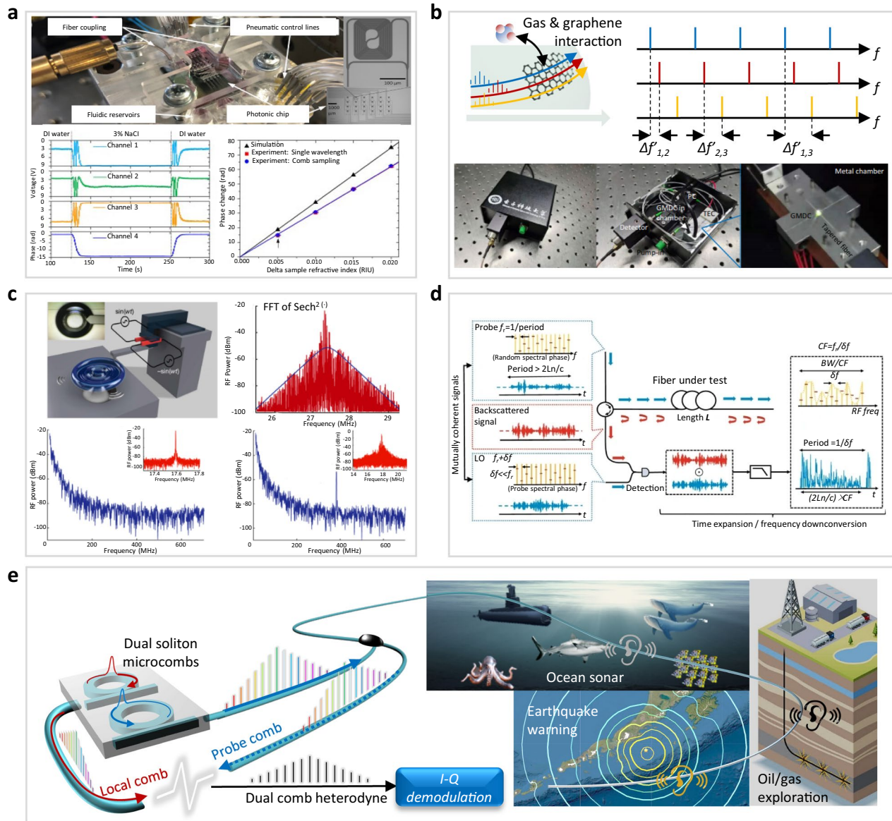
Fig. 12 Microcomb based sensing applications. a , Optical frequency comb based photonic refractive index sensor [233]. b , Multispecies and individual gas molecule detection using microcomb solitons in a graphene over-modal microresonator [95]. c , Detection of a low-frequency vibration of a cantilever tip using optomechanical soliton microcomb in a microtoroid [237]. d , Dual EO microcomb source enhances spatial resolution in a fiber distributed sensing system [238]. e , On-chip dual Kerr microcomb based ultrasensitive distributed acoustic sensor [240]
