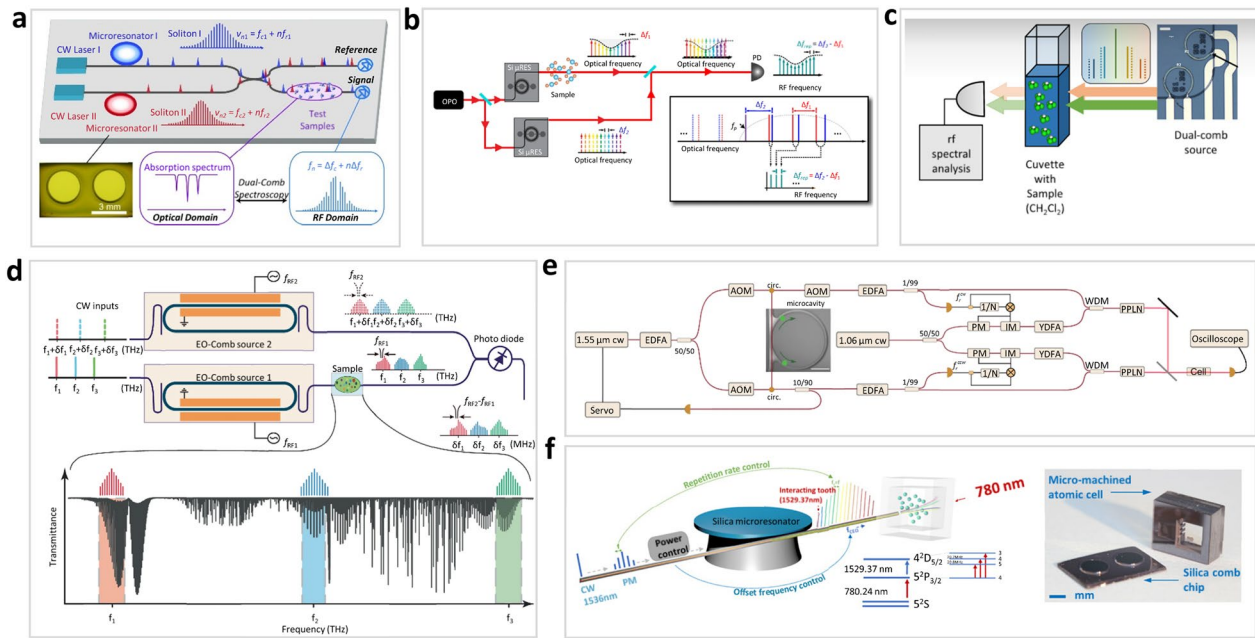
Fig. 10 Microcomb based spectroscopy. a , Microcomb-based dual-comb spectroscopy [212]. b , Silicon-chip-based mid-infrared dual-comb spectroscopy [213]. c , On-chip dual-comb source spectroscopy [83]. d , Active microcomb atomic spectrometer, using two EO microcombs [214]. e , microcomb-based GHz-midinfrared dual-comb spectroscopy [215]. f , Atomic spectroscopy with Kerr microcomb [216]
